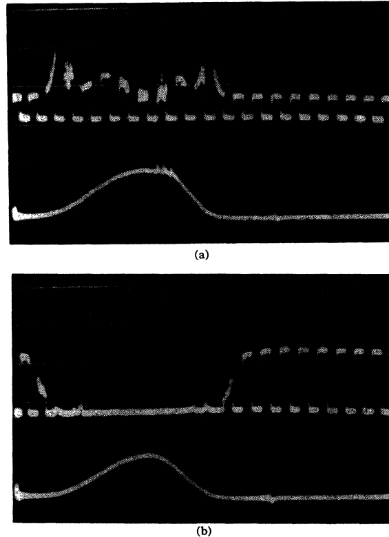
FIG. 4. Oscillograms showing (a) microwave signals transmitting through a plasma parallel to the magnetic field and (b) microwave signals attenuated by a plasma. In both (a) and (b) the lower trace is the current through the discharge.
